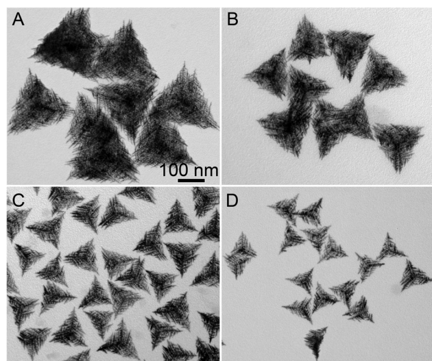
Figure 4. TEM images of Pt–Cu HTBNFs obtained through the addition of different amounts of KI aqueous solution in the synthesis while keeping the other parameters constant: A) 30 \mu\text{L} , B) 50 \mu\text{L} , C) 100 \mu\text{L} , and D) 150 \mu\text{L} . The scale bar in (A) also applies to (B–D).
